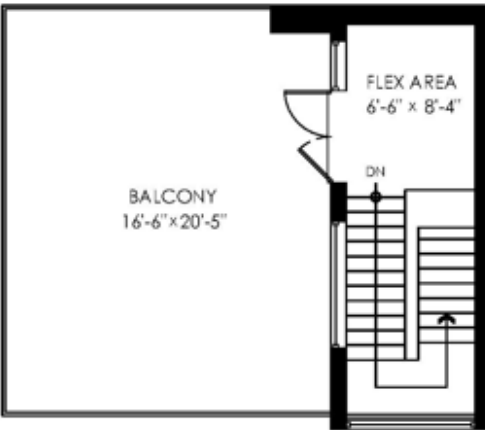
Top Floor Plan Floor Area: 167 sq.ft. Ceiling Height: 8'-1"
