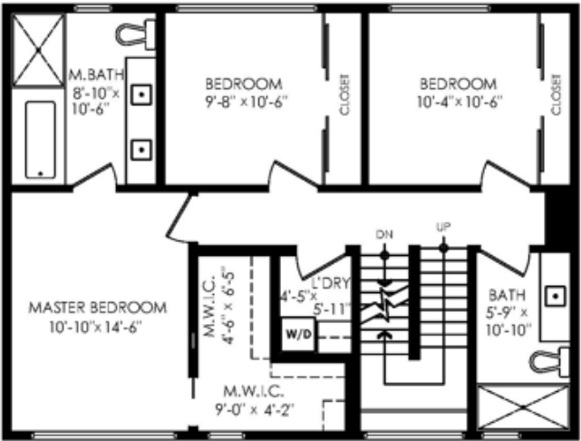
Upper Floor Plan Floor Area: 926 sq.ft. Ceiling Height: 8'-1"
