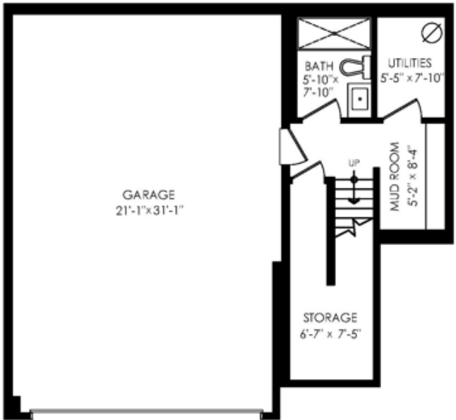
Lower Floor Plan Floor Area: 343 sq.ft. Ceiling Height: 8'-7"
