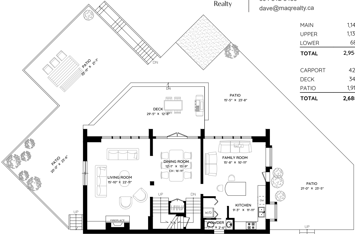
MAIN FLOOR 1,143 SQ.FT. CH: 8'-0"
